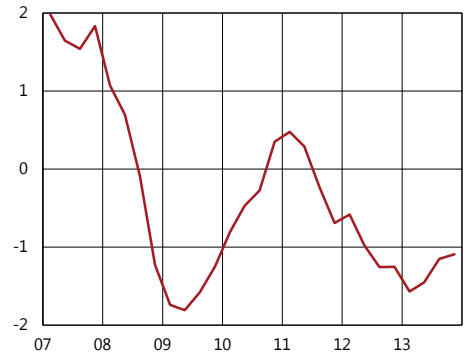
Diagram 2:5. RU-indikatorn Standardavvikelse
