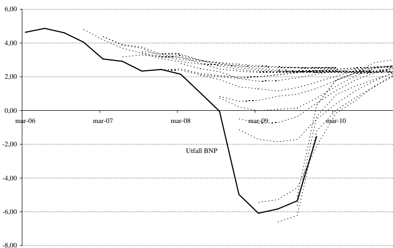
Diagram 18 Riksbankens BNP-prognoser
