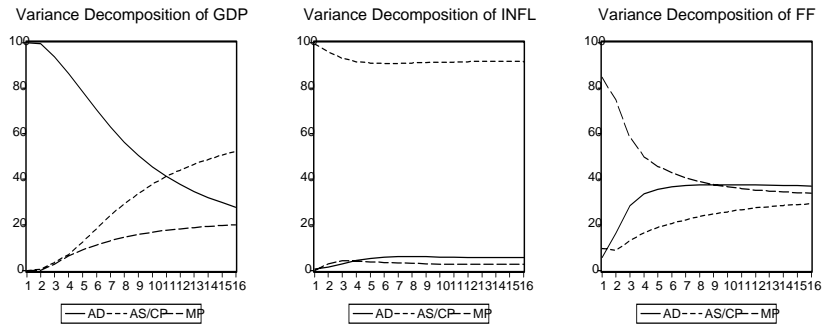
Figure 5: Variance decomposition for the misspecified VAR.
